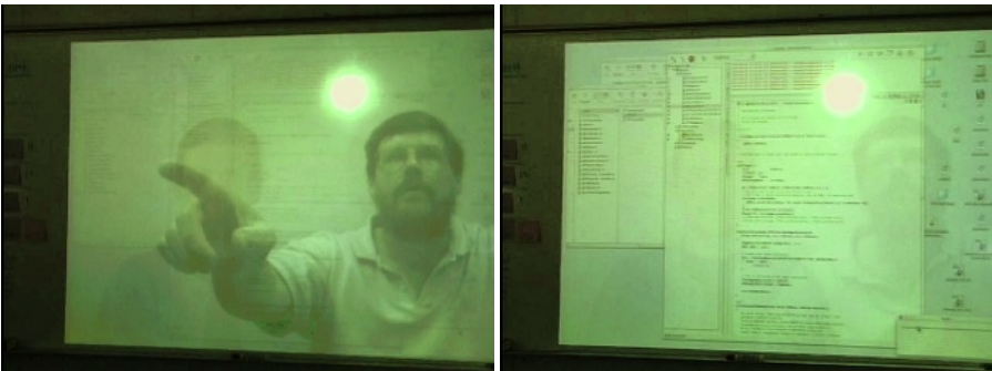
Fig. 5. Varying levels of transparency in dual-head Facetop
